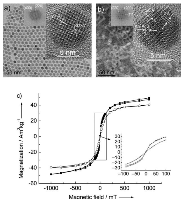
Figure 1. TEM and HRTEM images, as well as FFT patterns of HRTEM of Fe 3 O 4 NCs coated with a) oleic acid and b) PMAO-graft-PNIPAAm copolymer, negatively stained with ammonium molybdate (2 wt %); c) room-temperature magnetization curve of as-synthesized Fe 3 O 4 NCs (■) and Fe 3 O 4 NCs coated with PMAO-graft-PNIPAAm (○).
